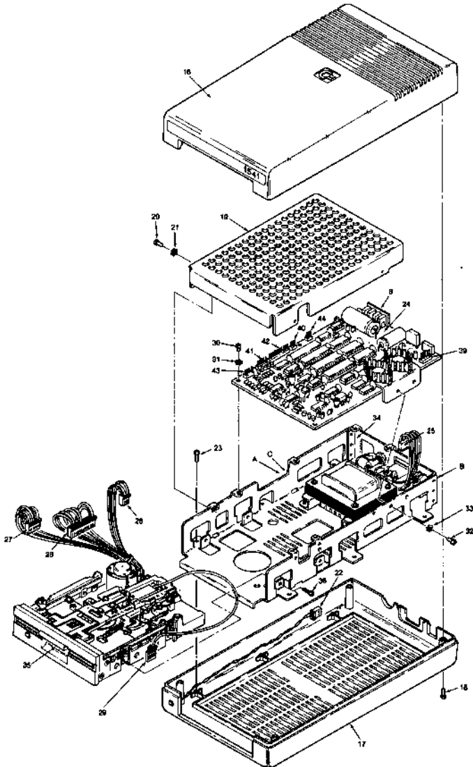
Fig. 1-17. Reassembly of Model 1541.
